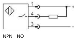
NPN NO
