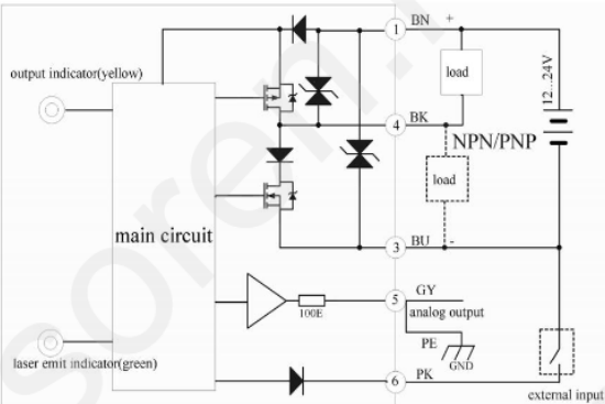
Analog output
