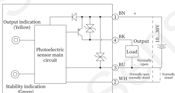
PNP
