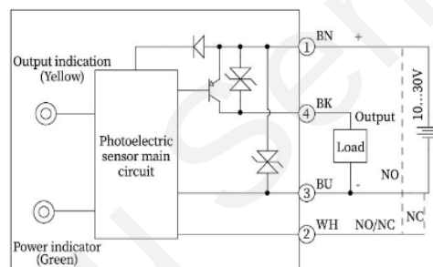
PNP
